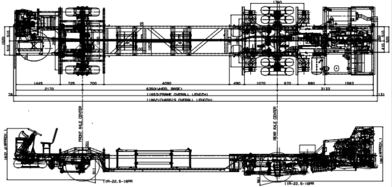
BH117KH (RHD) CHASSIS LAYOUT FOR THAILAND
